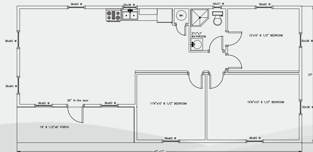
24'x48' WEEKENDER CABIN with 6' wide porch (985 sa ft)
