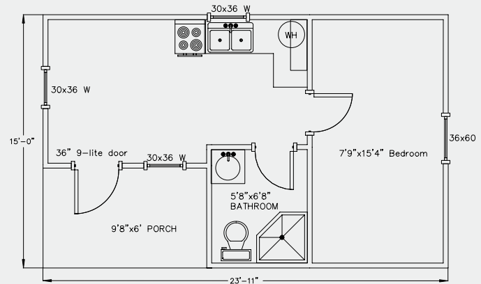
16x24 WEEKENDER CABIN with 6' Porch (300 sq. ft)
