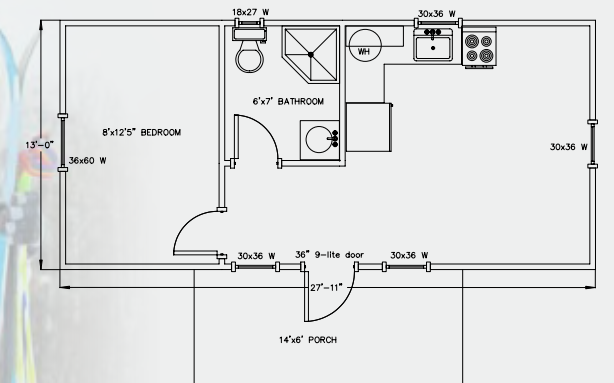
14'x28' KEUKA CABIN with 6' wide porch (364 sq. feet)
