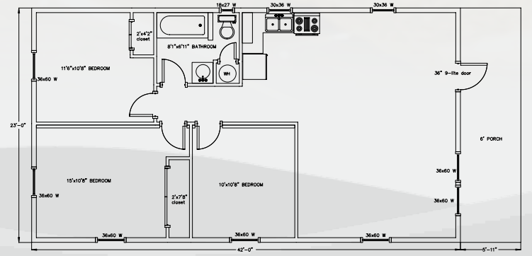
24'x48' ADIRONDACK CABIN with 6' wide porch (966 sq. feet)
