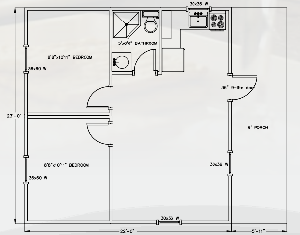
24'x28' ADIRONDACK CABIN with 6' wide porch (506 sq. feet)
