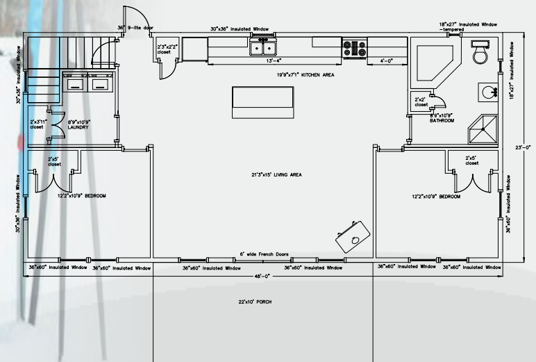
24'x48' KEUKA CABIN with 10' wide porch (1,104 sq. feet)
