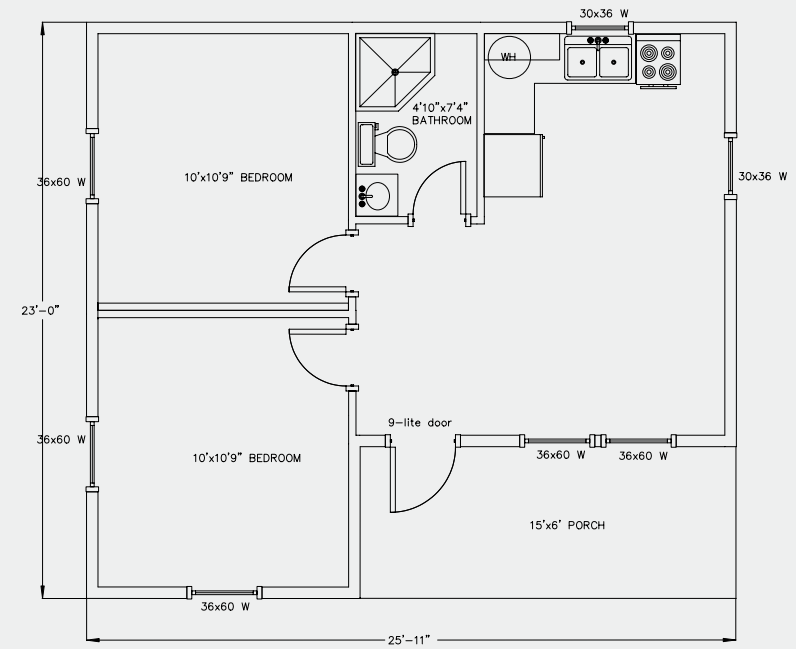
24'x26' WEEKENDER CABIN with 6' wide porch (508 sq ft)
