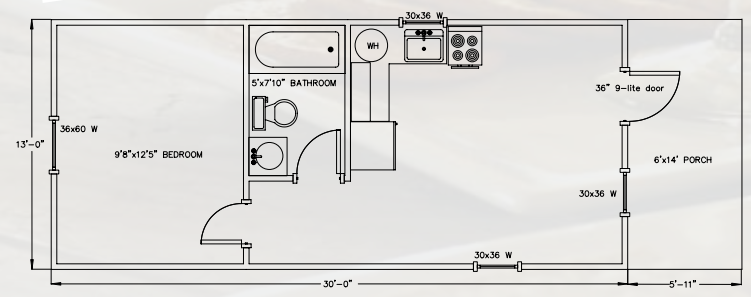
14'x36' ADIRONDACK CABIN with 6' wide porch (390 sq. feet)
